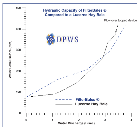
Hydraulic Performance Chart
