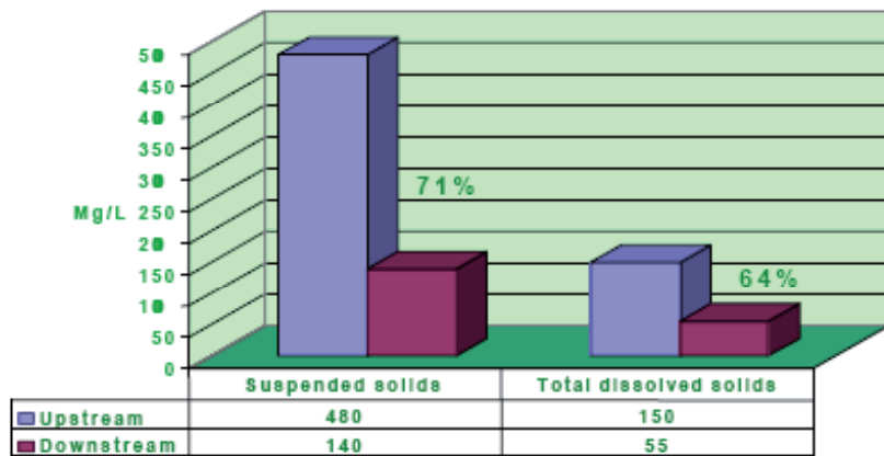
Sediment Removal Performance Chart
